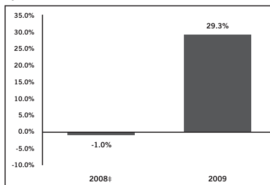
Cymbria, class J NAV returns
