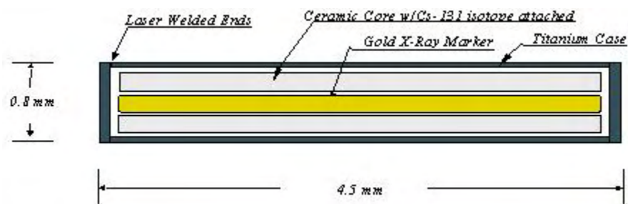
Figure 1: Cross section of ^{131}\text{Cs} seed
