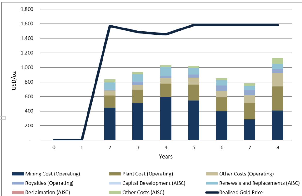
Figure 6: ASIC cost on Yearly Basis TGME Underground Project
