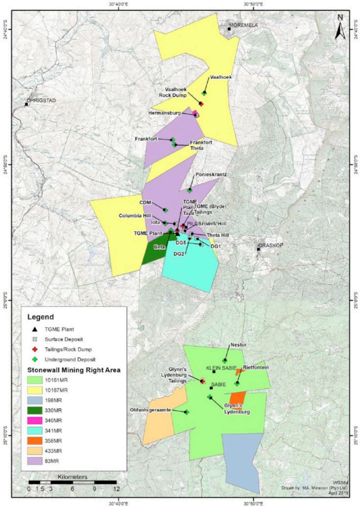
Figure 7: Tenement map
